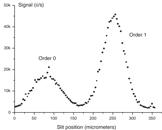
FIG. 2: Laser diffraction of the lithium beam : number of atoms detected per second as a function of the x -position (in \mu\text{m} ) of the detector slit S_D (counting period : 1 s). Two peaks are observed, corresponding to the diffraction orders 0 and +1. In this experiment, only one laser standing wave, associated to mirror M_2 , is present. We have verified the absence of a peak corresponding to the order -1, in agreement with the theoretical prediction for Bragg regime. A few noise bursts of the Langmuir-Taylor hot wire detector are visible.
